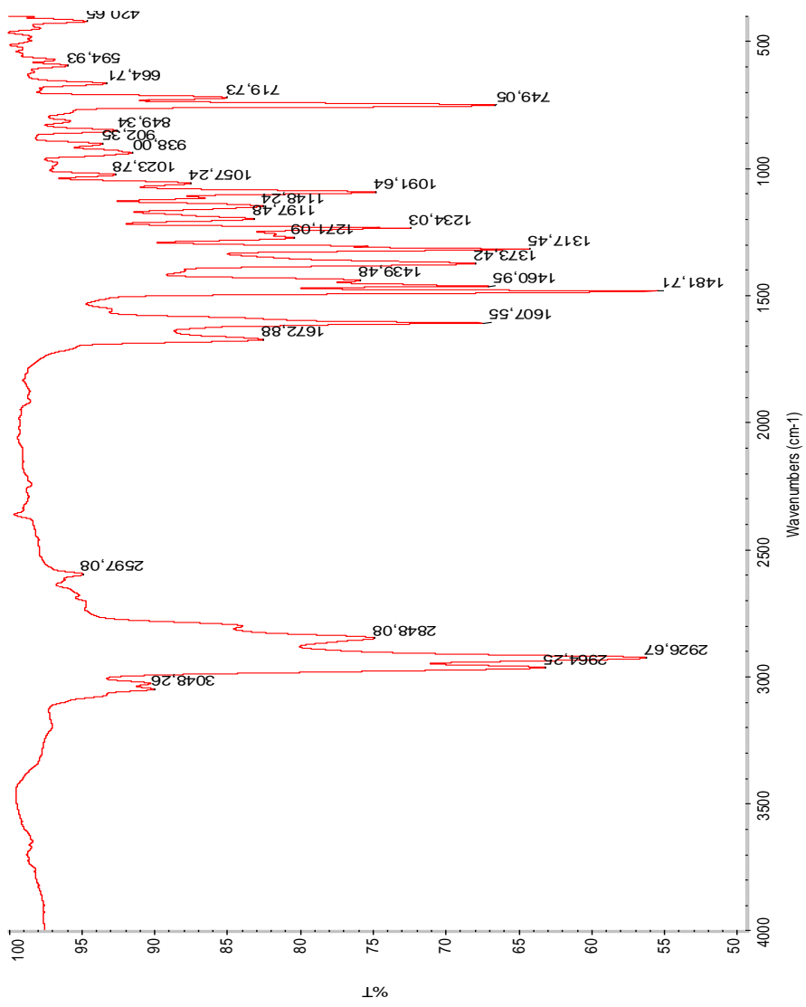
Figure 41: IR spectrum of (AZ-2).
